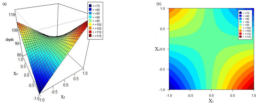
Fig. 5. A Response surface plot, frequency and pumping current
