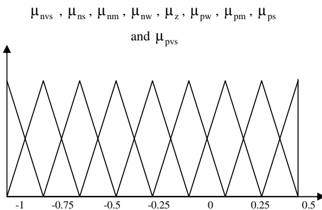
Fig. 3. Membership functions
