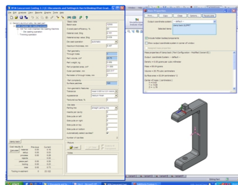
Fig. 6. DFM Concurrent Costing in Use
