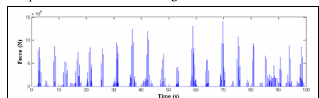
Fig 12. Amplitude of contact force for \Omega = 5.725 rad/s (axial-lateral)
