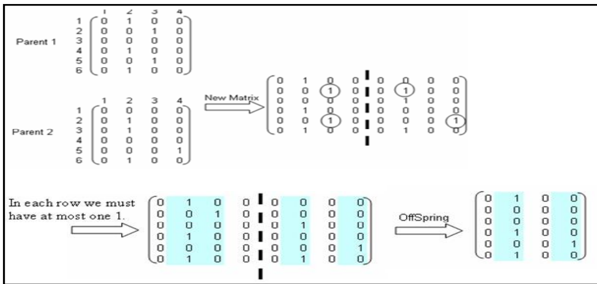
Fig. 4. Sample of crossover operator in GA
