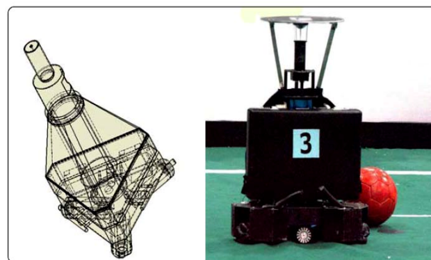
Fig. 1. Our robot is a 3-wheeled omni-directional mobile robot with an omni-directional vision system, a normal camera and a kicking device, and is controlled by a notebook PC.
