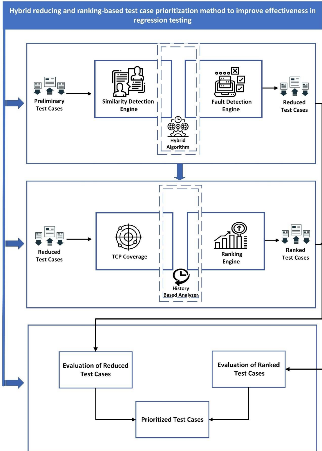
Fig. 2. Hybrid framework
