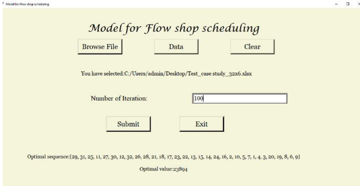
Fig. 7. Output window
