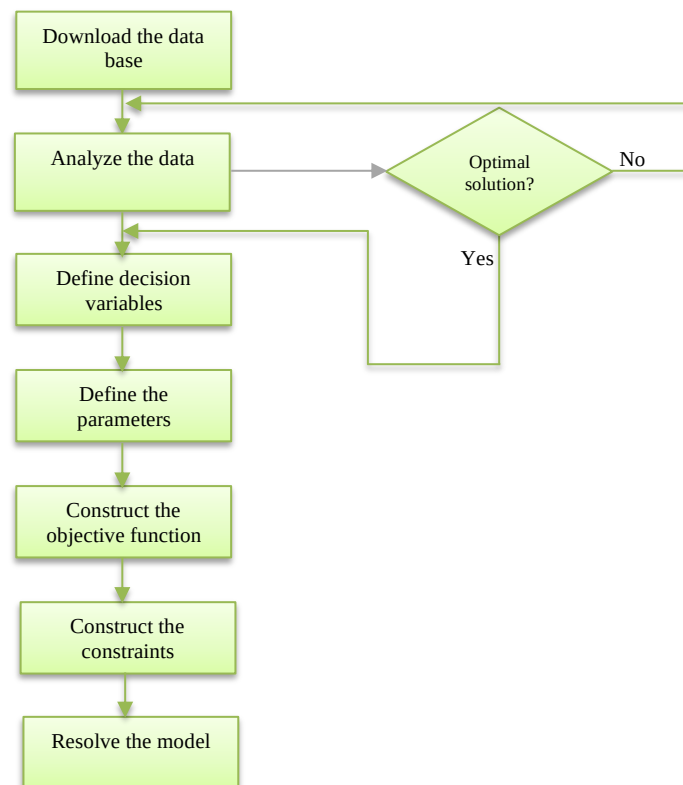
Fig. 9. Program operation algorithm in PYTHON
