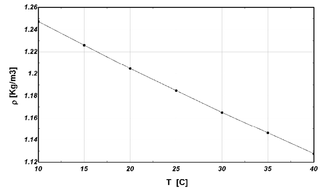
Fig. 6. Effect of temperature on density of air [23]
