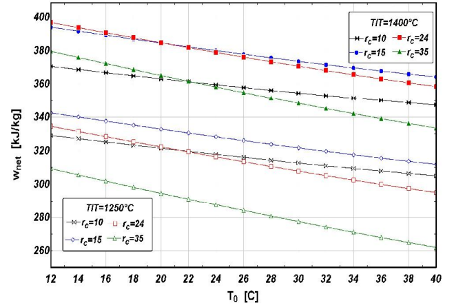
Fig. 2. Effect of compressor inlet air temperature on SGT specific work in different r_c and TIT ( \phi=60\% )
