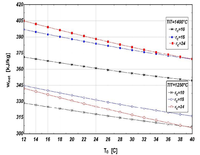
Fig. 3. Effect of compressor inlet air temperature on RGT specific work in different r_c and TIT ( \phi=60\% )
