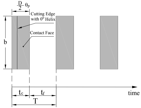
Fig. 3. Contact face, cutting time t_c and non cutting time t_f for 0° helix
