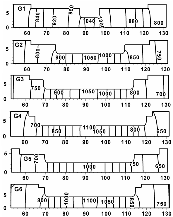
Fig. 7. Temperature distribution in G1, G2, G3, G4, G5, and G6 deformed at 1000°C and \omega=3 \text{ rad.sec}^{-1}
