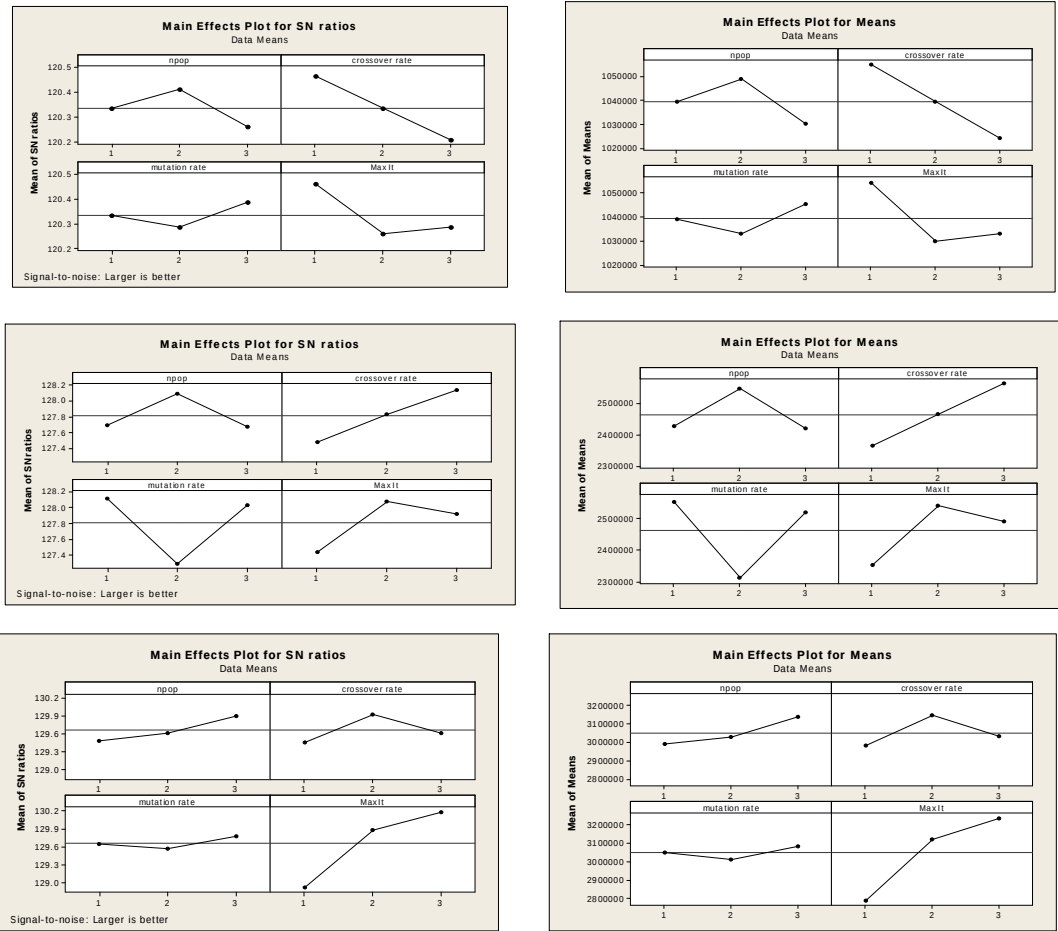
Fig. 8. Taguchi analysis
