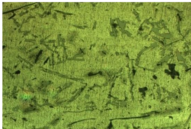
Fig. 5. Al 2124 microstructure after etching.
