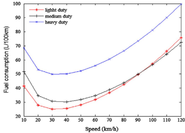
Fig. 1. The fuel consumption of each type of vehicles at different speeds
