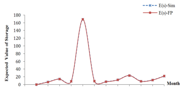
Fig. 3. The evaluation of optimal FP policy by simulation for case 2; Expected Value of Storage.
