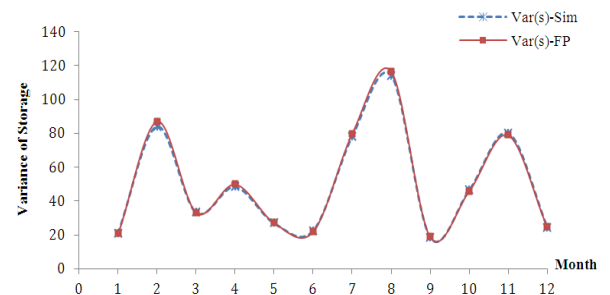
Fig. 4. The evaluation of optimal FP policy by simulation for case 2; Variance of Storage.
