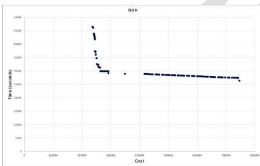
Figure A3. NHH Pareto front for 30LL under Model I
