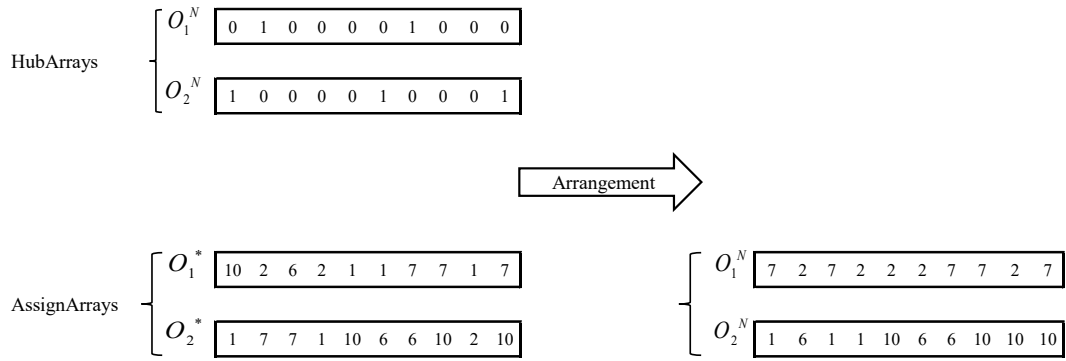
Figure 4. Example of offspring arrangement in NHR (adapted from Topcuoglu et al. [12])
