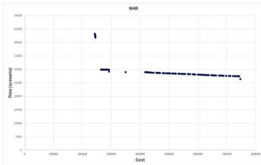
Figure A2. NHR Pareto front for 30LL under Model I
