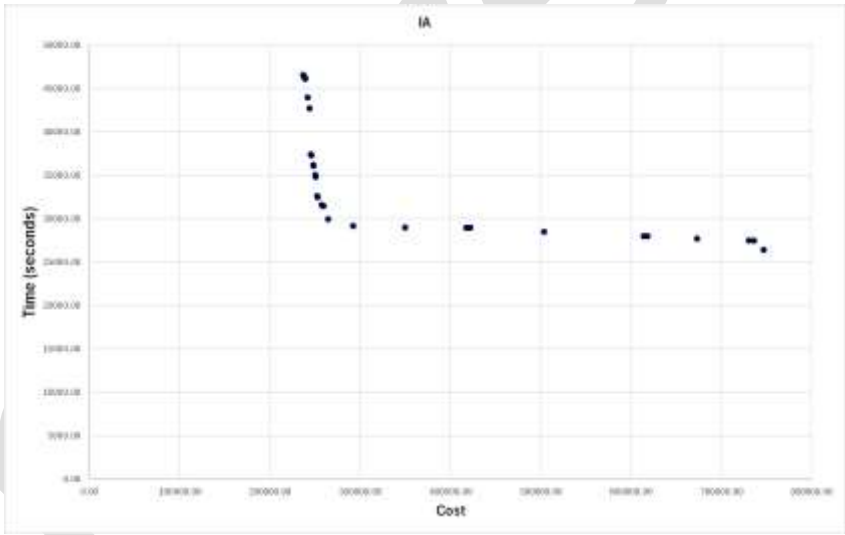
Figure A1. IA Pareto front for 30LL under Model I
