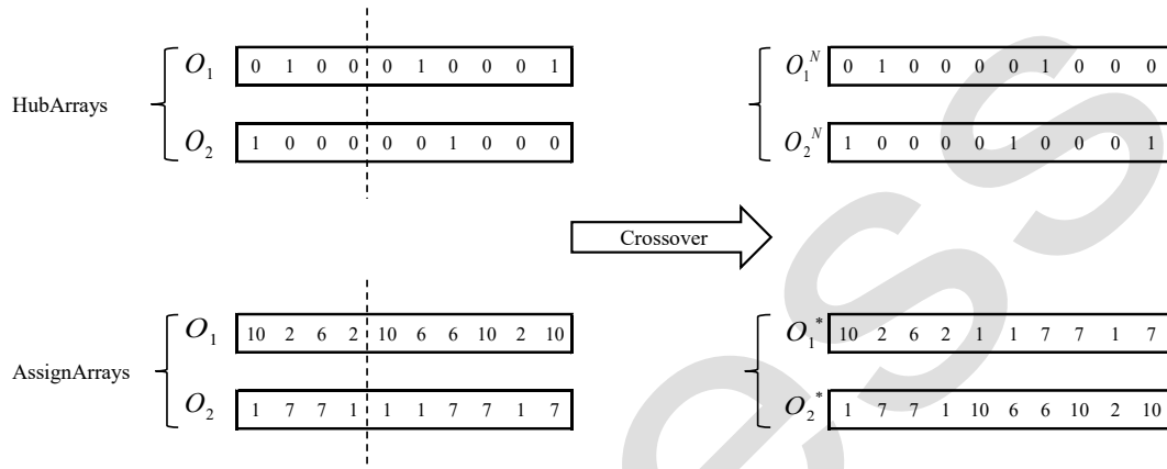
Figure 3. Example of single-point crossover (adapted from Topcuoglu et al. [12])
