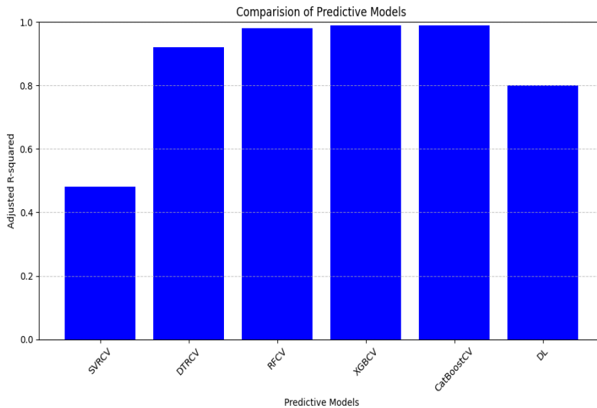
Fig. 10. Algorithm comparison.
