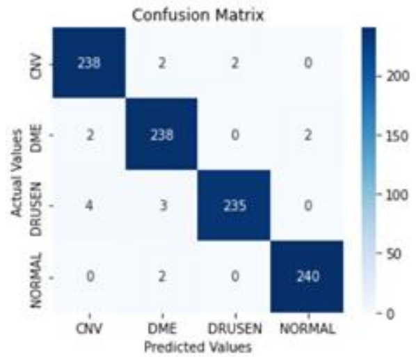
(b) ResNet-50V2
