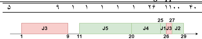
Fig. 9. Scheduling five jobs for example1
