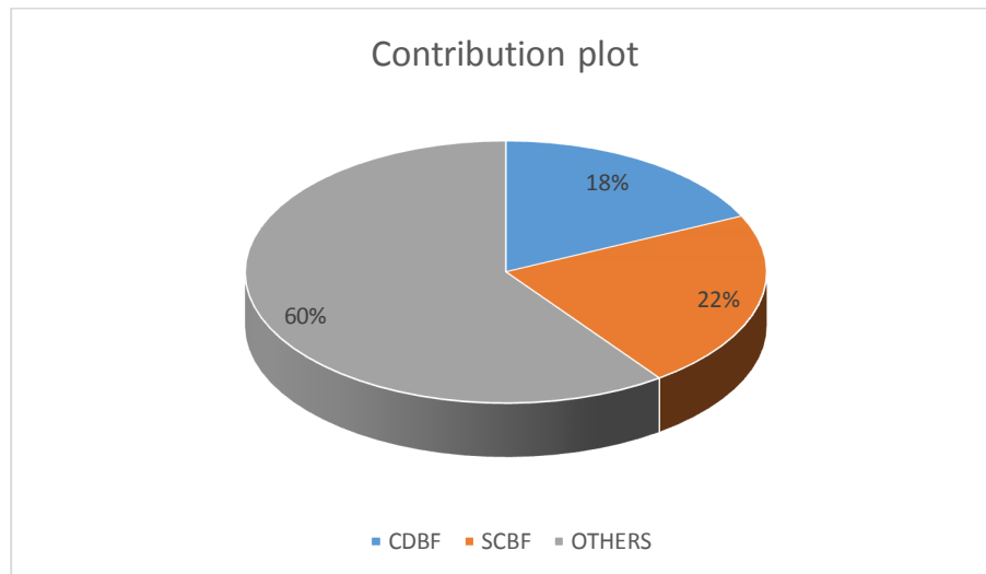
Fig. 5. (c) Contribution plot of out-of-control observation no 31
