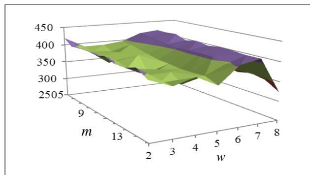
Fig. 2. Residual trends of m and w for enrollments of the University of Alabama
