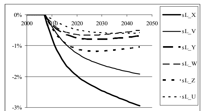
Fig. 5. Variations for wage indexes at production sectors
