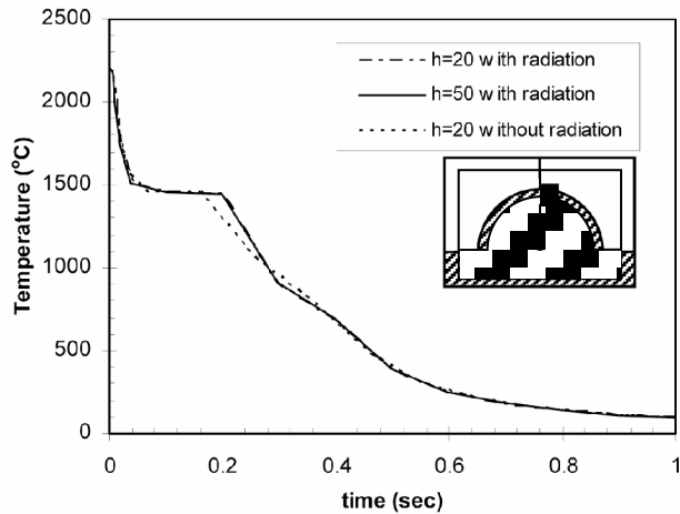
Fig. 13. Boundary effects on the cooling curve of a point on the droplet
