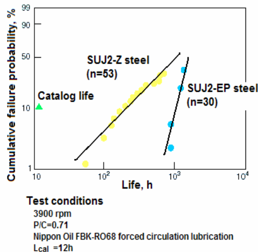
Fig. 1. Rolling Contact Fatigue Life of Deep Groove Ball Bearings (6206) made of SUJ2-EP on Radial Type Test rig.
