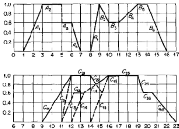
Fig. 4. Method of Dubois and Prade for fuzzy addition of two non-convex fuzzy numbers [25]
