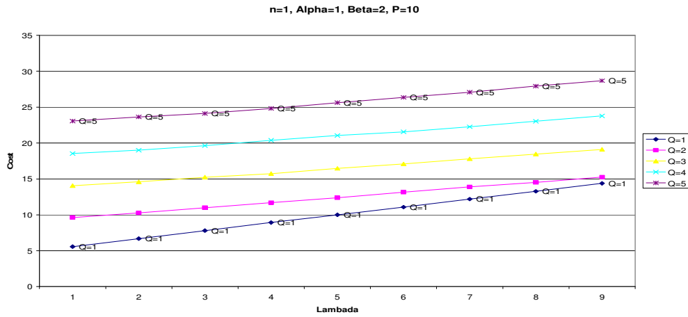
Fig. 4. Cost and Demand rate Interaction (n=1, Alpha=1, Beta=2, P=10)
