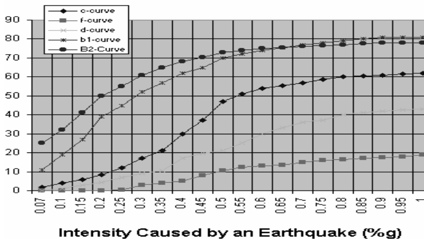
Fig 4. Fragility curve for different building types based on EMS intensity
